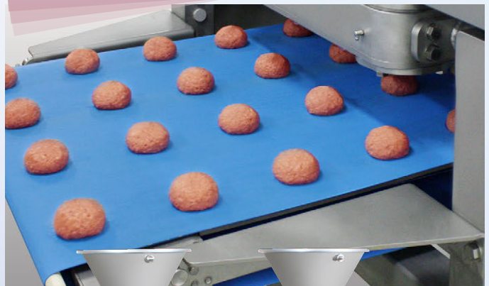
Four Rows Encrusting Model Producing 48,000 pcs / hour
